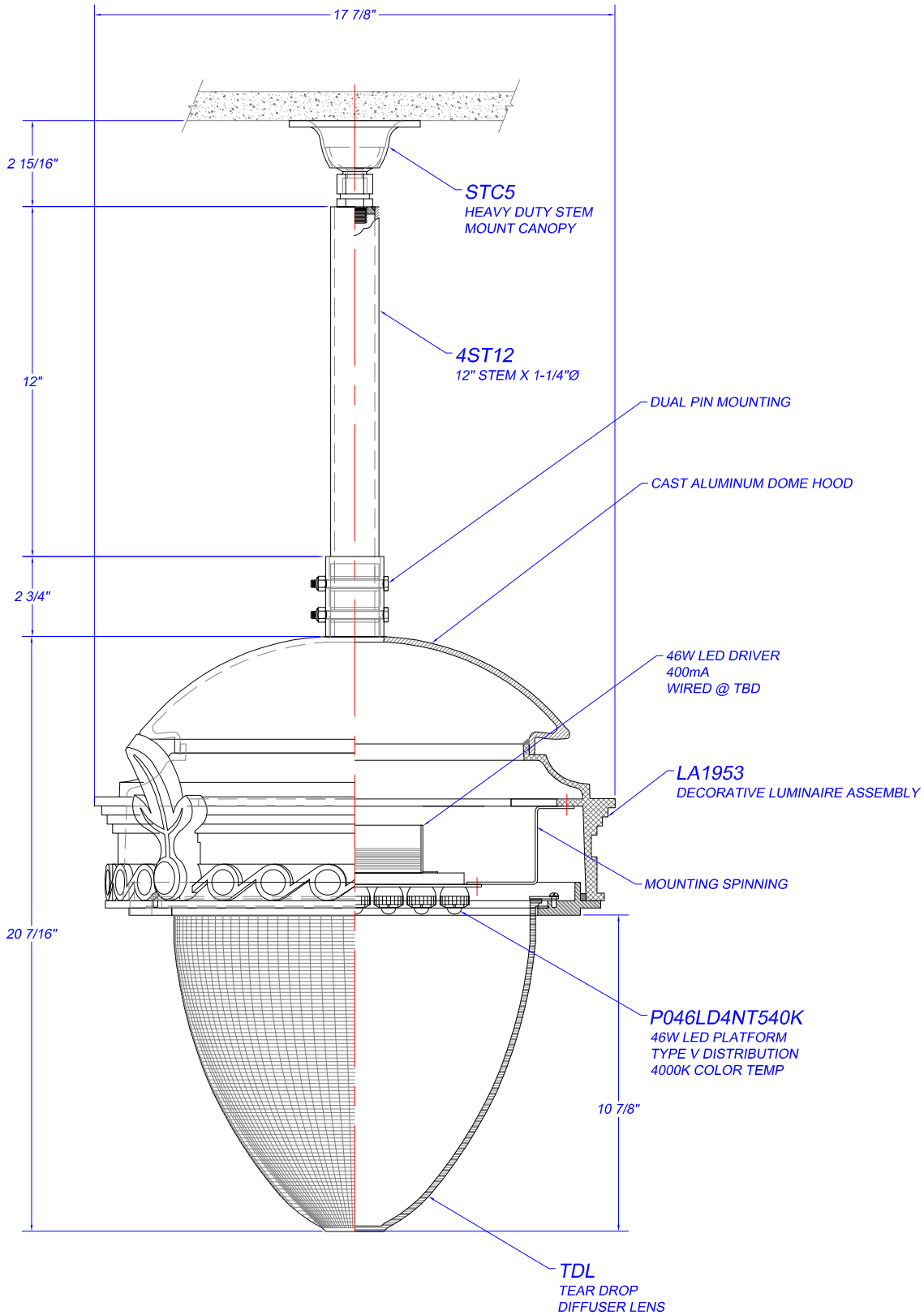
PROPORTIONAL VIEW
