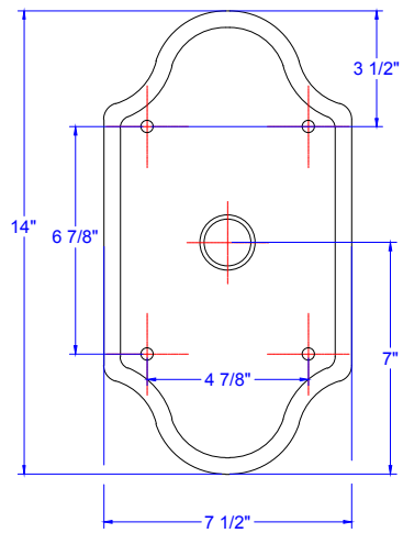
MOUNTING DETAIL
