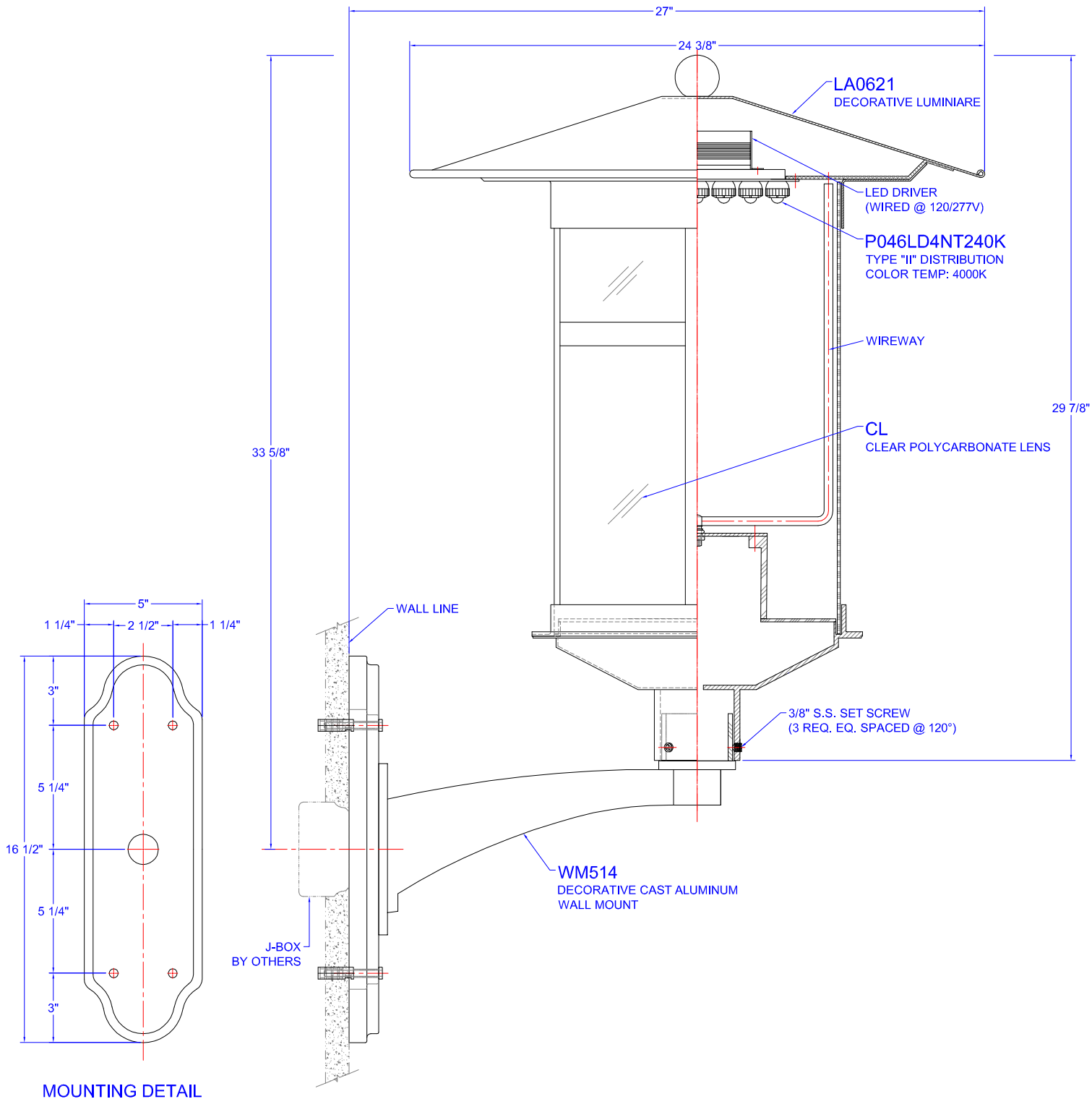
MOUNTING DETAIL
